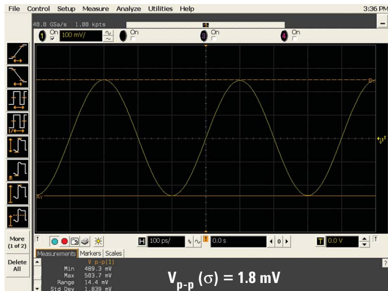
Figure 12b: 2.5-GHz sine wave captured on the Agilent Infiniium DSO80304B sampling at 40 GSa/s (interleaved)
