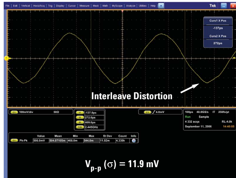
Figure 13b: 2.5-GHz sine wave captured on Tektronix DPO7254 2.5-GHz bandwidth oscilloscope sampling at 40 GSa/s (interleaved)
