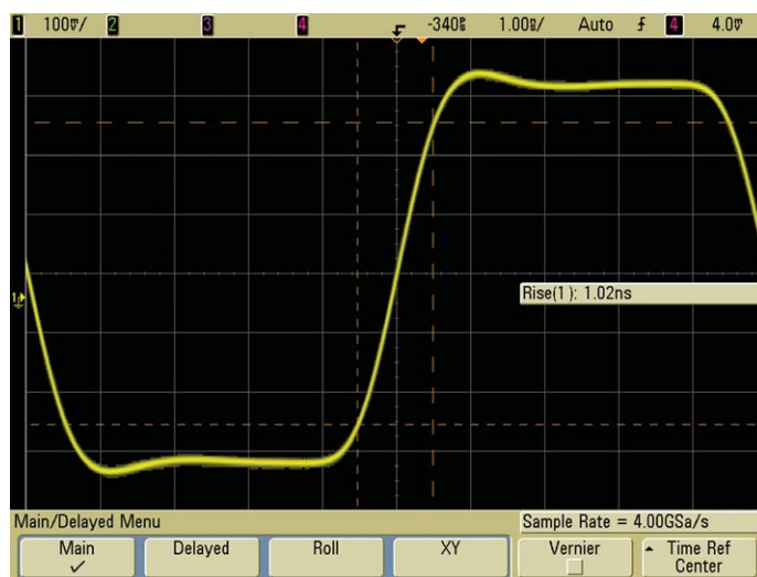
Figure 7: Agilent MSO6054A 500-MHz bandwidth scope sampling at 4 GSa/s produces minimal measurement improvement over sampling at 2 GSa/s
