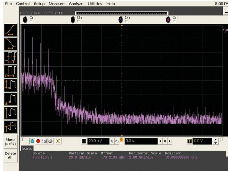
Figure 16a: FFT analysis on 400-MHz clock using an Agilent Infiniium DS080304B 3-GHz bandwidth oscilloscope
