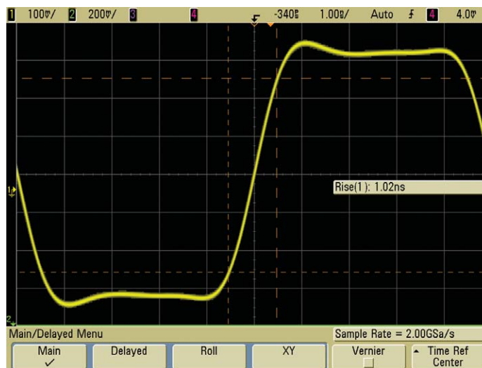
Figure 6: Agilent MSO6054A 500-MHz bandwidth scope sampling at 2 GSa/s shows an accurate measurement of this 100-MHz clock with a 1-ns edge speed
