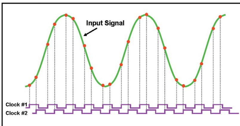
Figure 9: Timing diagram showing non-evenly spaced samples
