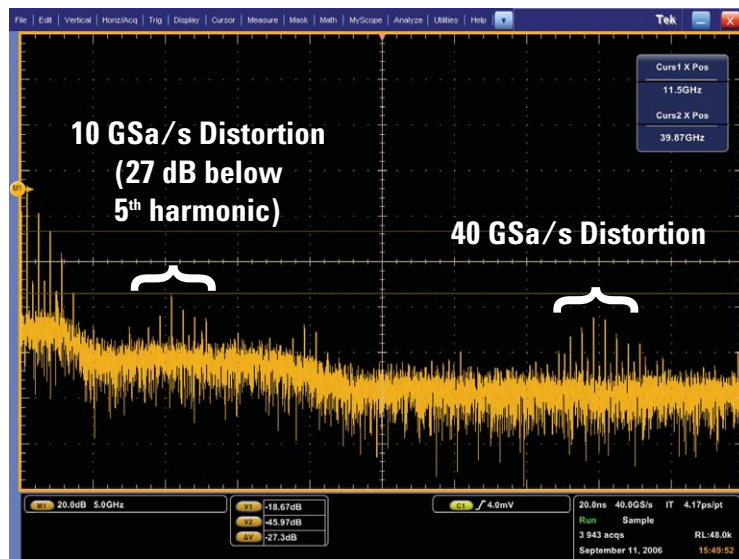
Figure 16b: FFT analysis on 400-MHz clock using a Tektronix DP07254 2.5-GHz bandwidth oscilloscope
