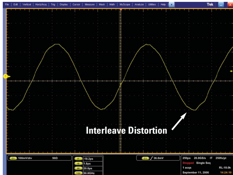
Figure 11b: 1-GHz sine wave captured on a Tektronix DPO7104 1-GHz bandwidth oscilloscope sampling at 20 GSa/s
