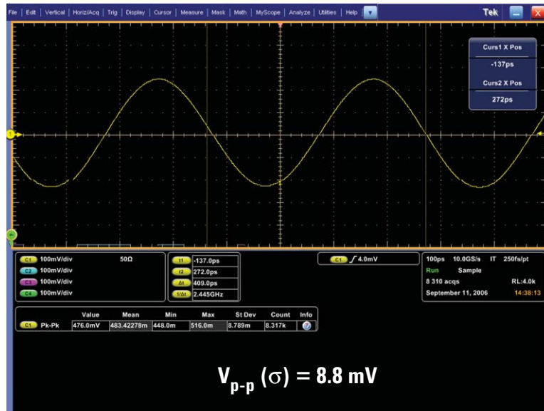
Figure 13a: 2.5-GHz sine wave captured on Tektronix DPO7254 2.5-GHz bandwidth oscilloscope sampling at 10 GSa/s (non-interleaved)
