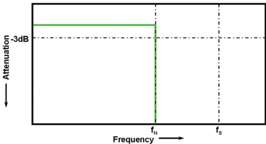
Figure 2: Theoretical brick-wall frequency response
